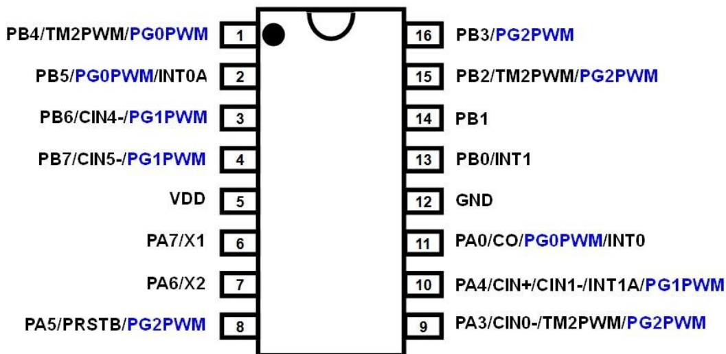
PTS152-S16 (SOP16-150mil)
