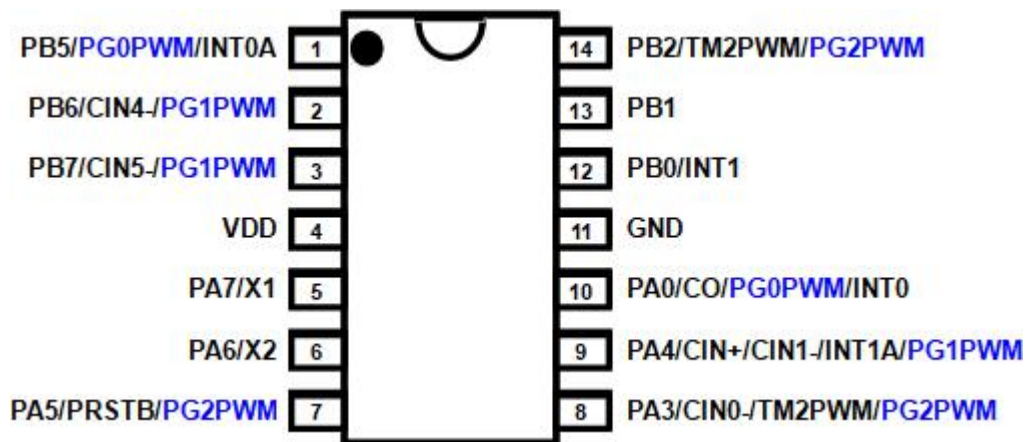
PTS152-S14 (SOP14-150mil)
