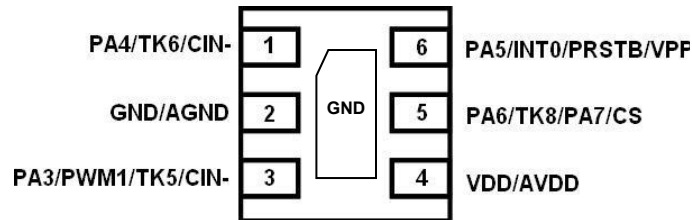
P3902: DFN6 (2*2mm)
