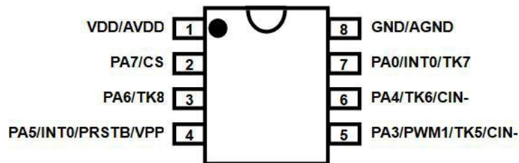
P3909: SOP8 (150mil) A
