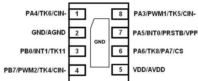
P3901: DFN8 (2*2mm)
