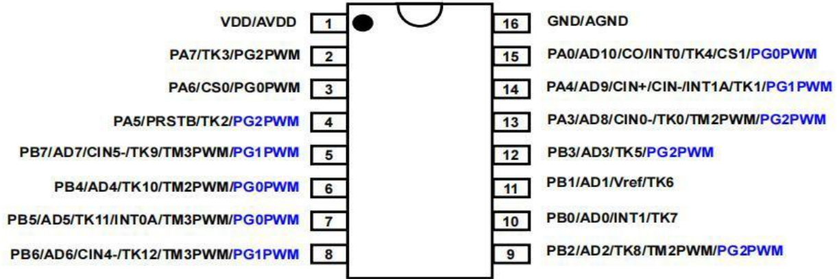
P3303 (SOP16A-150mil)
